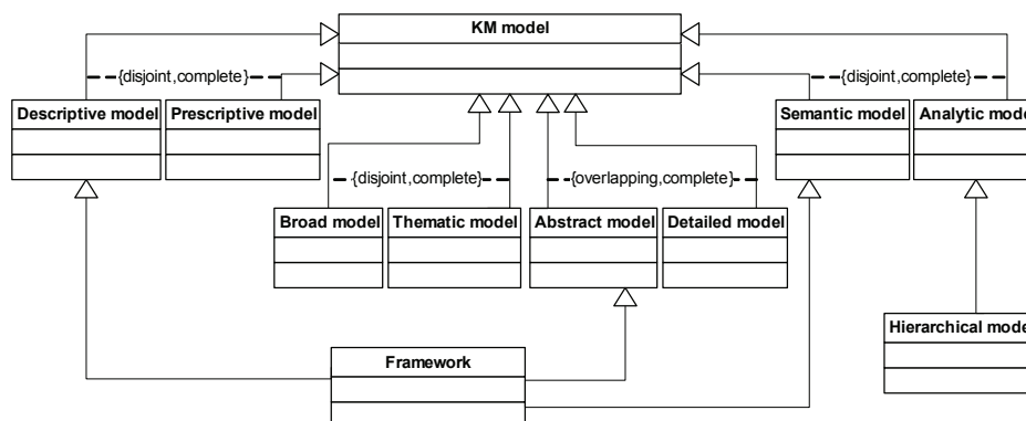
Figure 1. A classification of KM models
