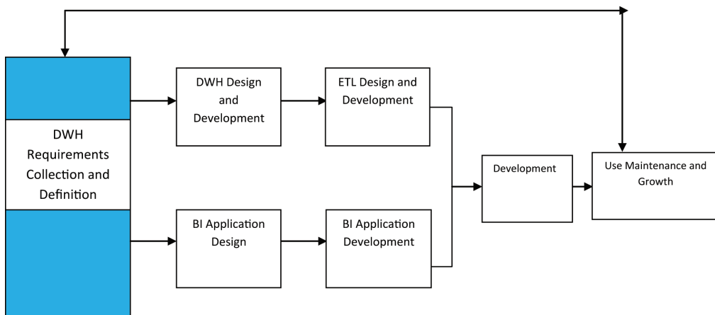
Figure 1. Abbreviated data warehouse system development lifecycle
