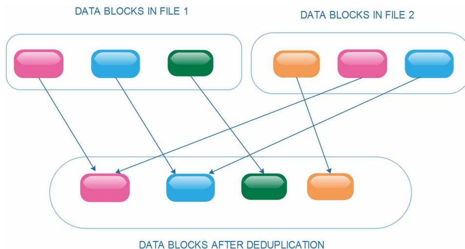
Figure 1. Data deduplication
