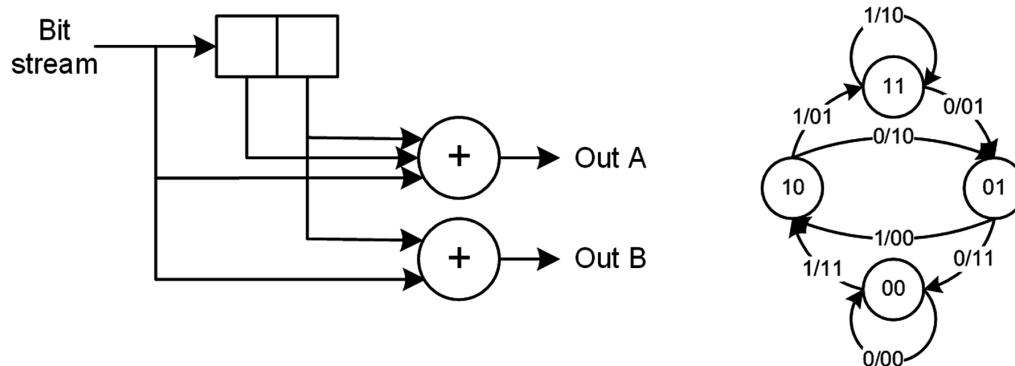
Figure 1. Convolution encoder with rate 1/2
