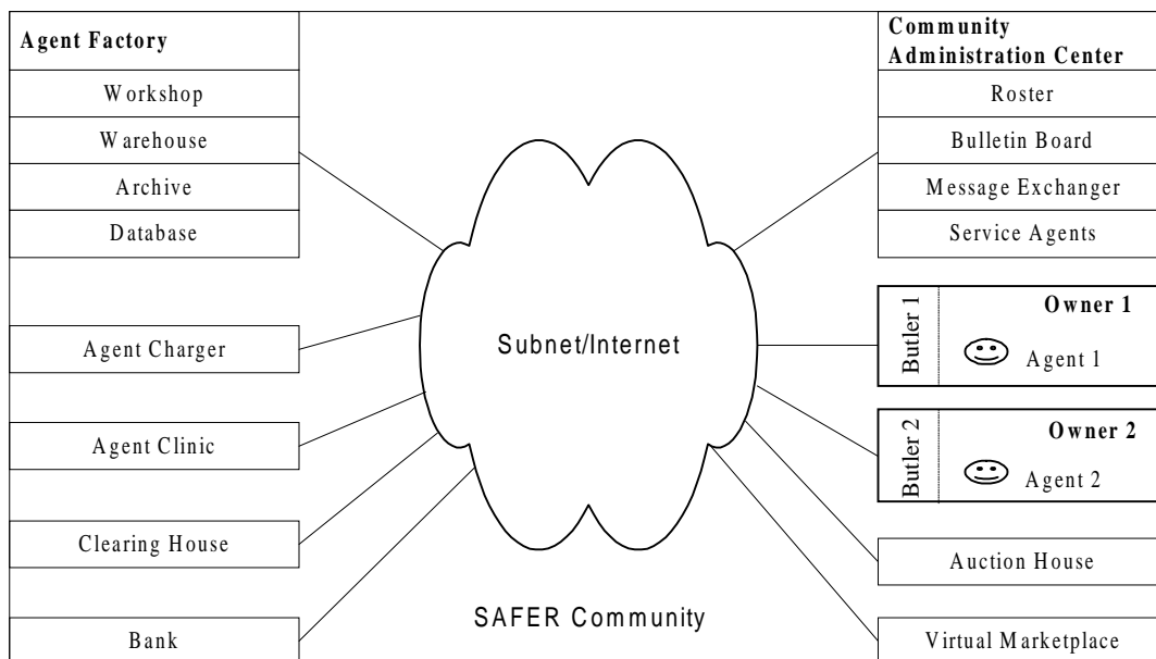
Figure 1. SAFER architecture
