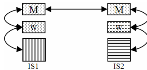
Figure 6. Mediation approach
