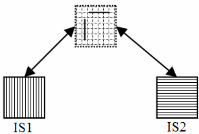
Figure 5. Ontology approach
