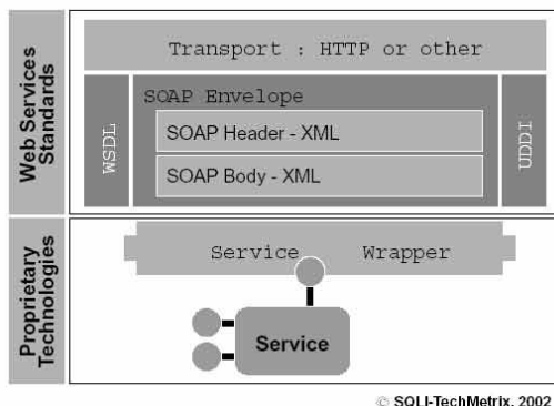
Fig 1: Web Service protocols and their relationships [IBM03]
