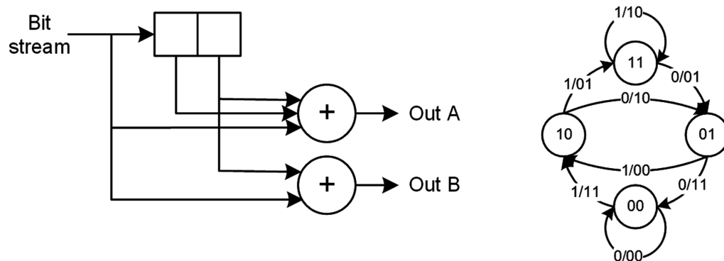
Figure 1. Convolution encoder with rate 1/2
