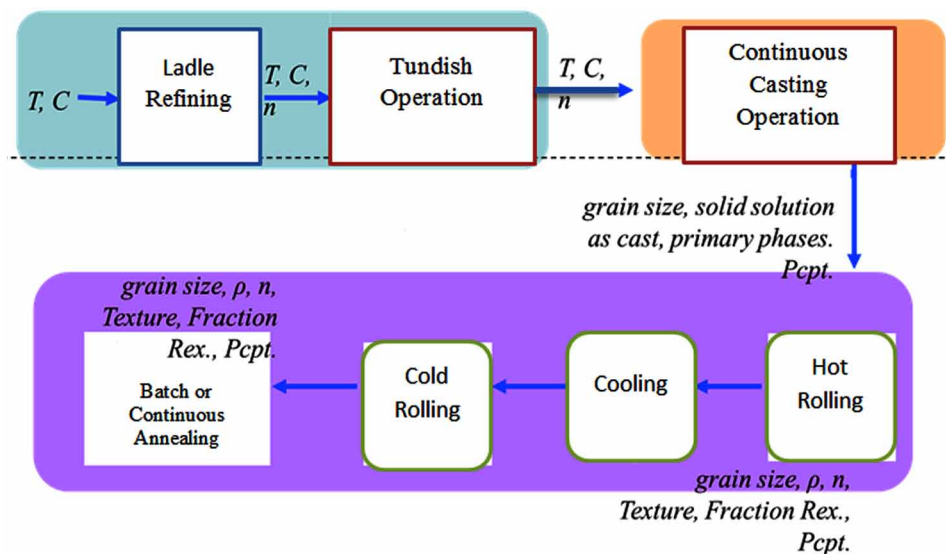
Figure 1. Steel product manufacturing chain
