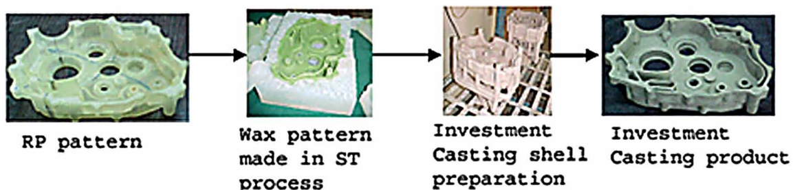
Figure 1. Development of metal components through RP-ST-wax pattern -investment casting
