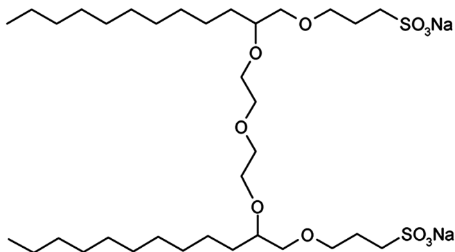
Figure 1. \alpha,\omega -trioxyethylene-bis(sodium 2-dodecyloxy-propylenesulfonate), an anionic gemini surfactant, used for preparation of niosomes Muzzalupo et al. 2008.
