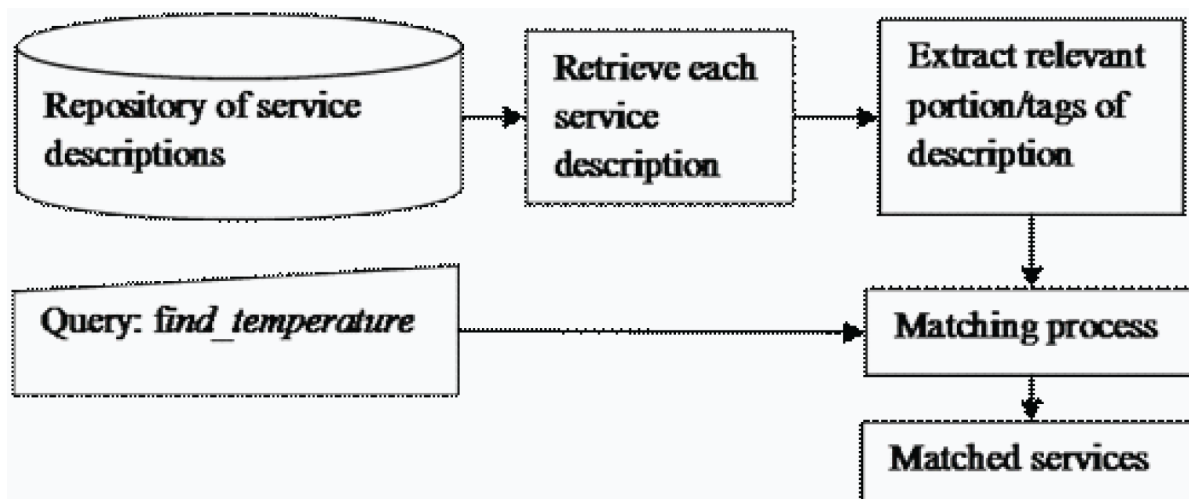
Figure 1. Process of service discovery
